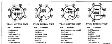
FIGURE 24.— Tube base connections.
