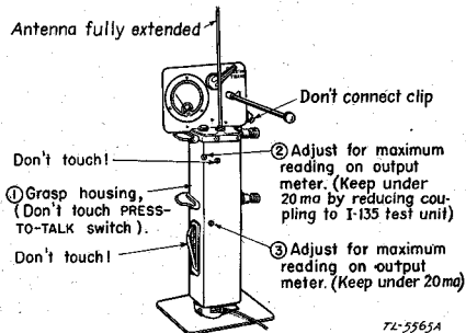
FIGURE 11.—Receiver presetting adjustments.
