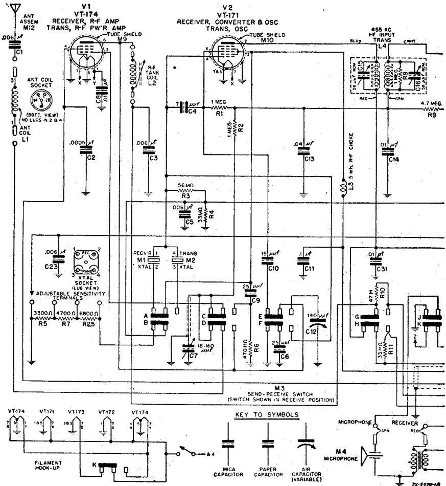
FIGURE 16.—Radio receiver and transmitter BC-611-A—schematic diagram.
