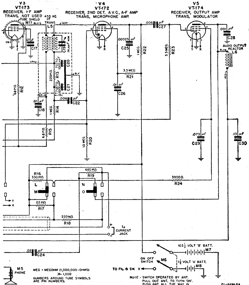
FIGURE 16.—Radio receiver and transmitter BC-611-A—schematic diagram—Continued.
